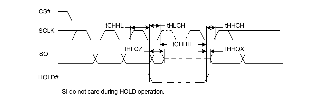
Figure43. Hold Timing
