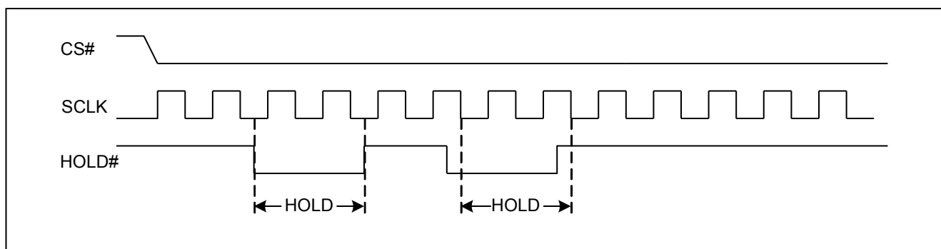
Figure 1. Hold Condition
